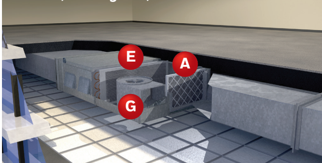
Air Filter, Cooling Coil, and Fan/Blower
